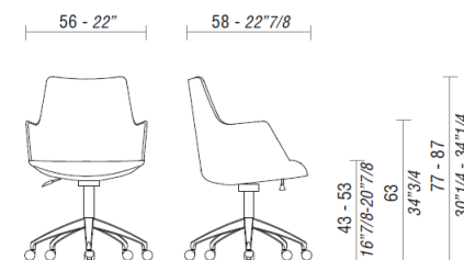
DIVINA, chair with star base.
