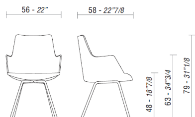
DIVINA, chair with 4 legs.
