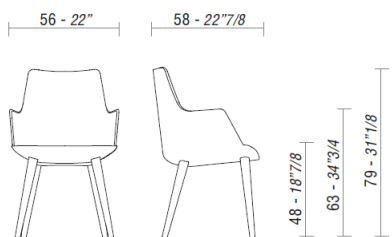
DIVINA, chair with 4 wooden legs.
