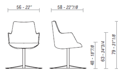
DIVINA, chair with swivel 4 star base.
