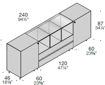
Container W240 (2 W60 modules + 1 W120 module)
