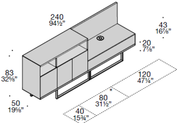
Sideboard W240 (94"1/4) with hinged doors and TV stand with front flap
