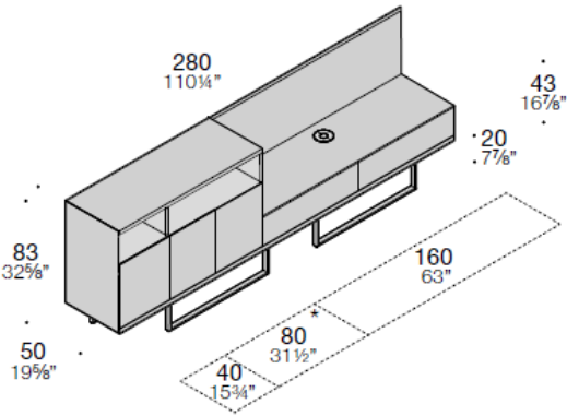
Sideboard W280 (110"1/4) with hinged doors and TV stand with front flap
