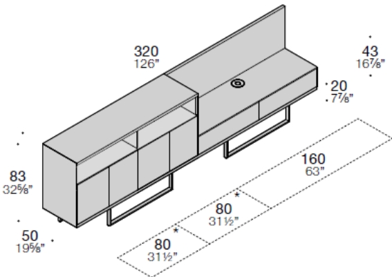
Sideboard W320 (126") with hinged doors and TV stand with front flap
