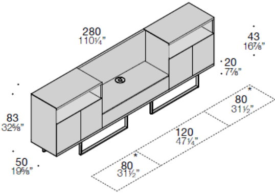
Sideboard W280 (110"1/4) with hinged doors and TV stand with front flap
