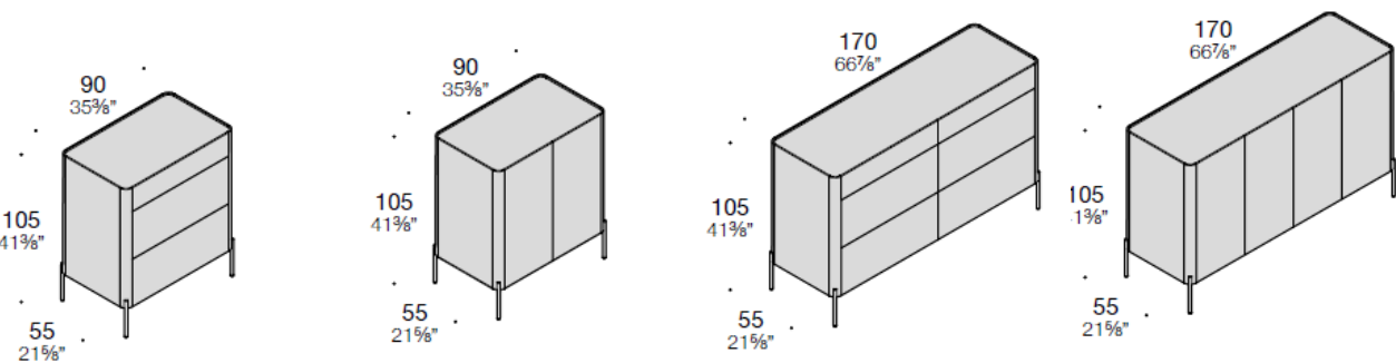
W90 (35"3/8) sideboard Madia with 2 filling cabinets and 1 drawer and with hinged doors
