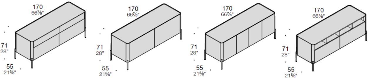
W170 (66"7/8) Sideboard Madia with 2 filling cabinets and 2 drawers, with 2 filling cabinets and internal drawer, with hinged doors and with 2 filling cabinets and open compartment.
