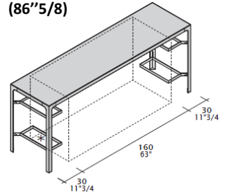
W 220 counter (86"5/8)
